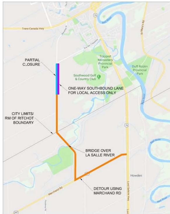
STAGE 2 (2019 CONSTRUCTION)
